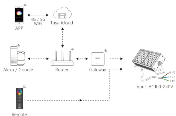
Application Diagram
