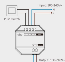
AC Triac Dimmer (TRI-C1)
