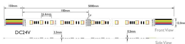
Dimensions(Unit: mm)
