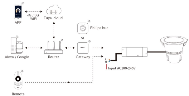
Application Diagram
