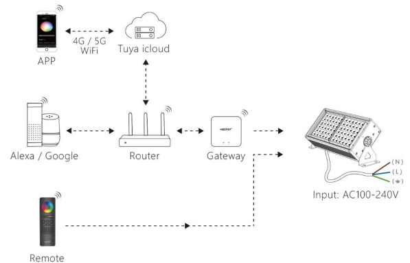
Application Diagram
