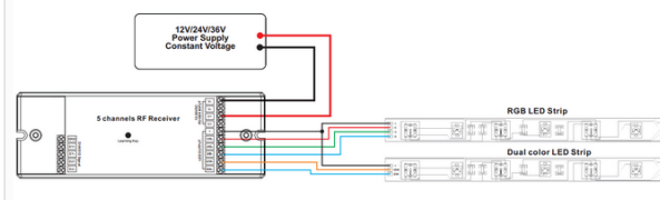
Wiring Diagram
