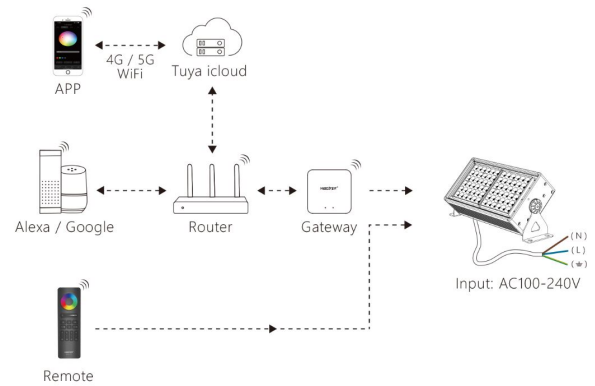
Application Diagram
