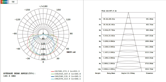
Luminous intensity distribution diagram
