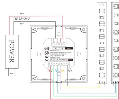
Diagram of connecting to LED strip
