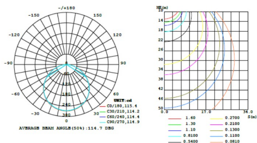
LUMINOUS INTENSITY DISTRIBUTION DIAGRAM
