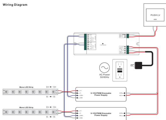
Wiring Diagram
