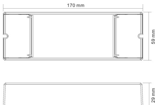
Product Dimension
